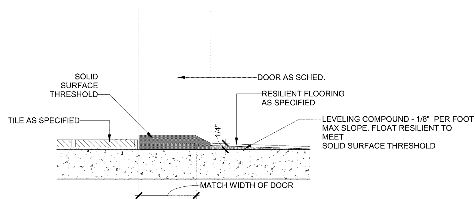
FLOORING TRANSITION - SOLID SURFACE THRESHOLD
