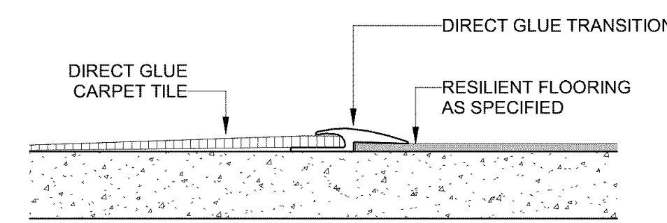
FLOORING TRANSITION - RESILIENT FLOORING TO CARPET
