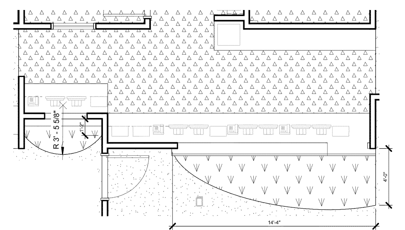
4 CHECK IN / CHECK OUT ENLARGED FINISH PLAN SCALE: 1/4" = 1'-0"
