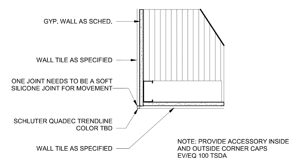
OUTSIDE TILE CORNER DETAIL
