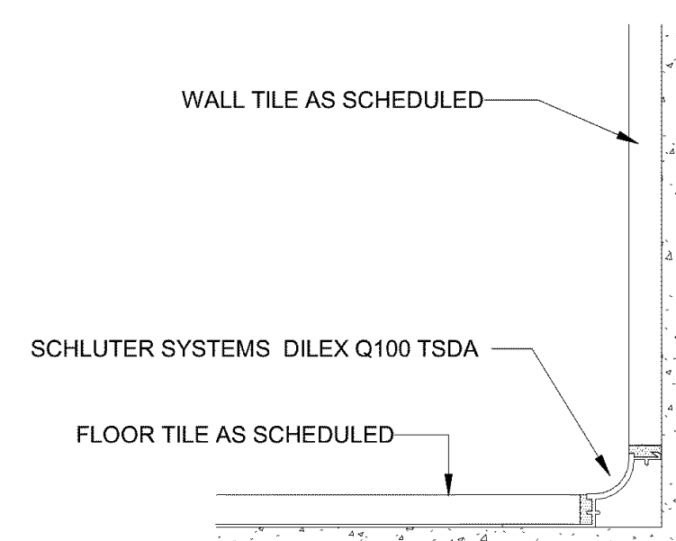
BASE TRANSITION - TILE FLOOR TO TILE WALL
