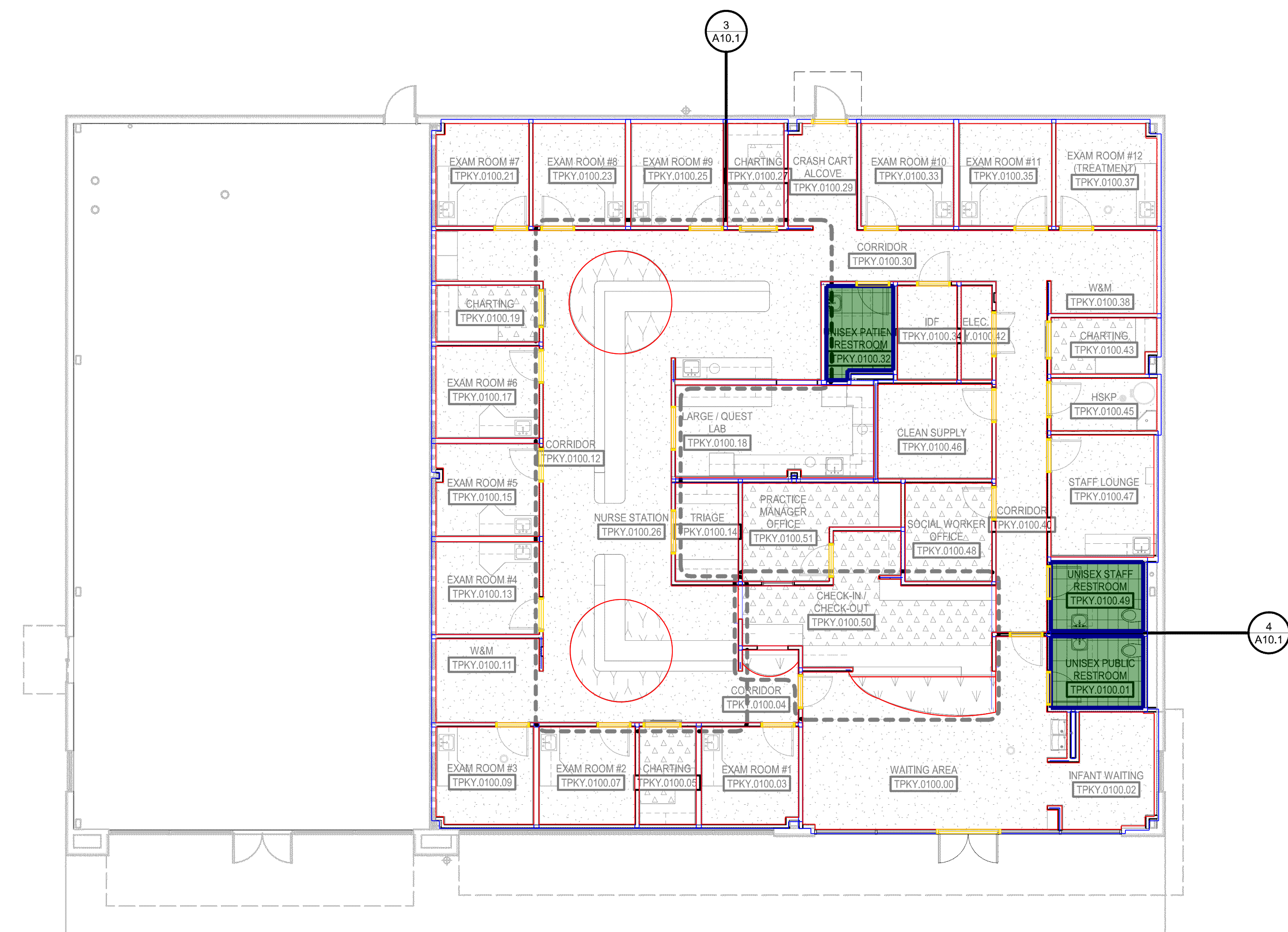
1 FIRST FLOOR FINISH PLAN SCALE: 1/8" = 1'-0"
