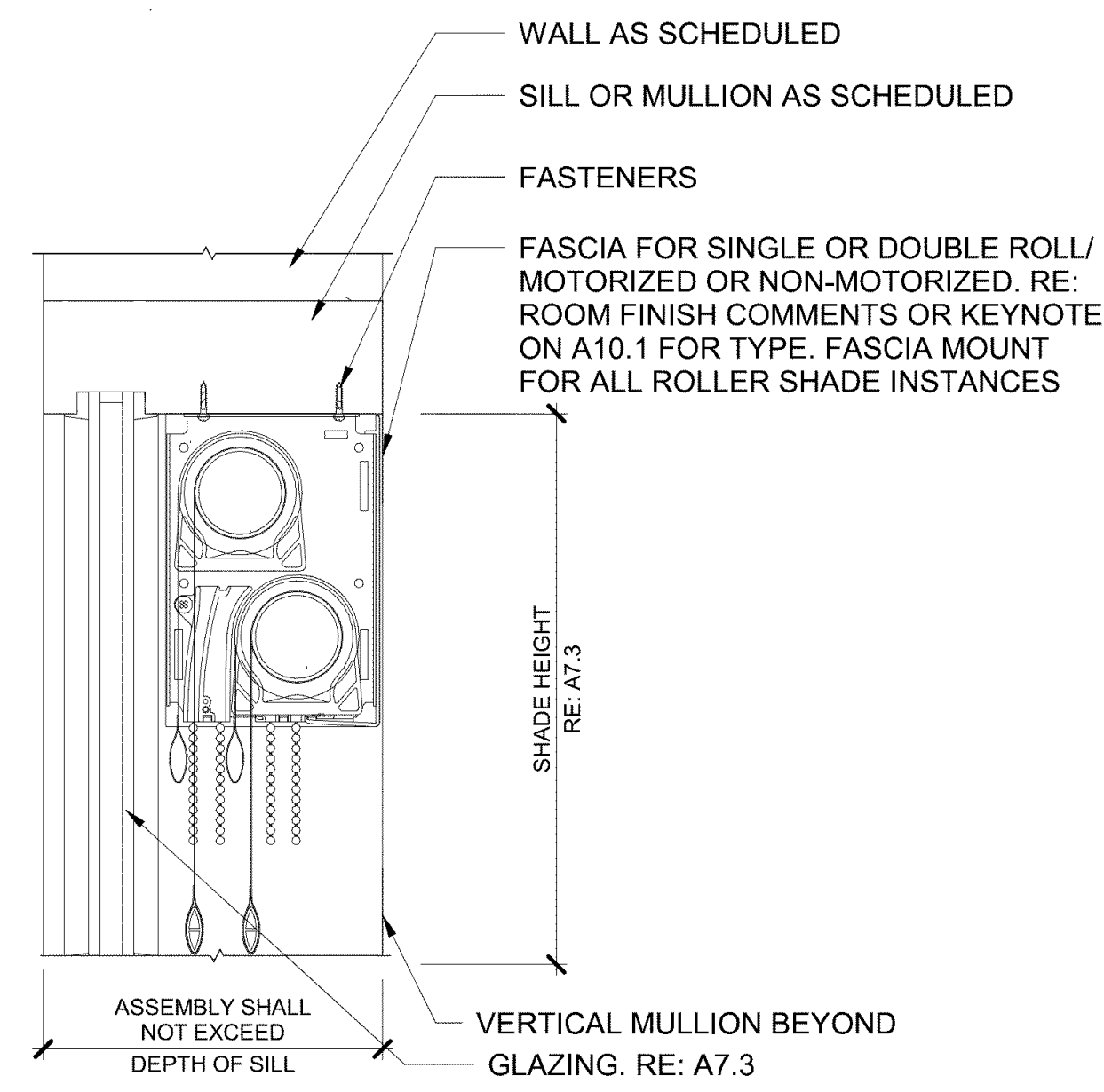
TYP. ROLLER SHADE DETAIL
