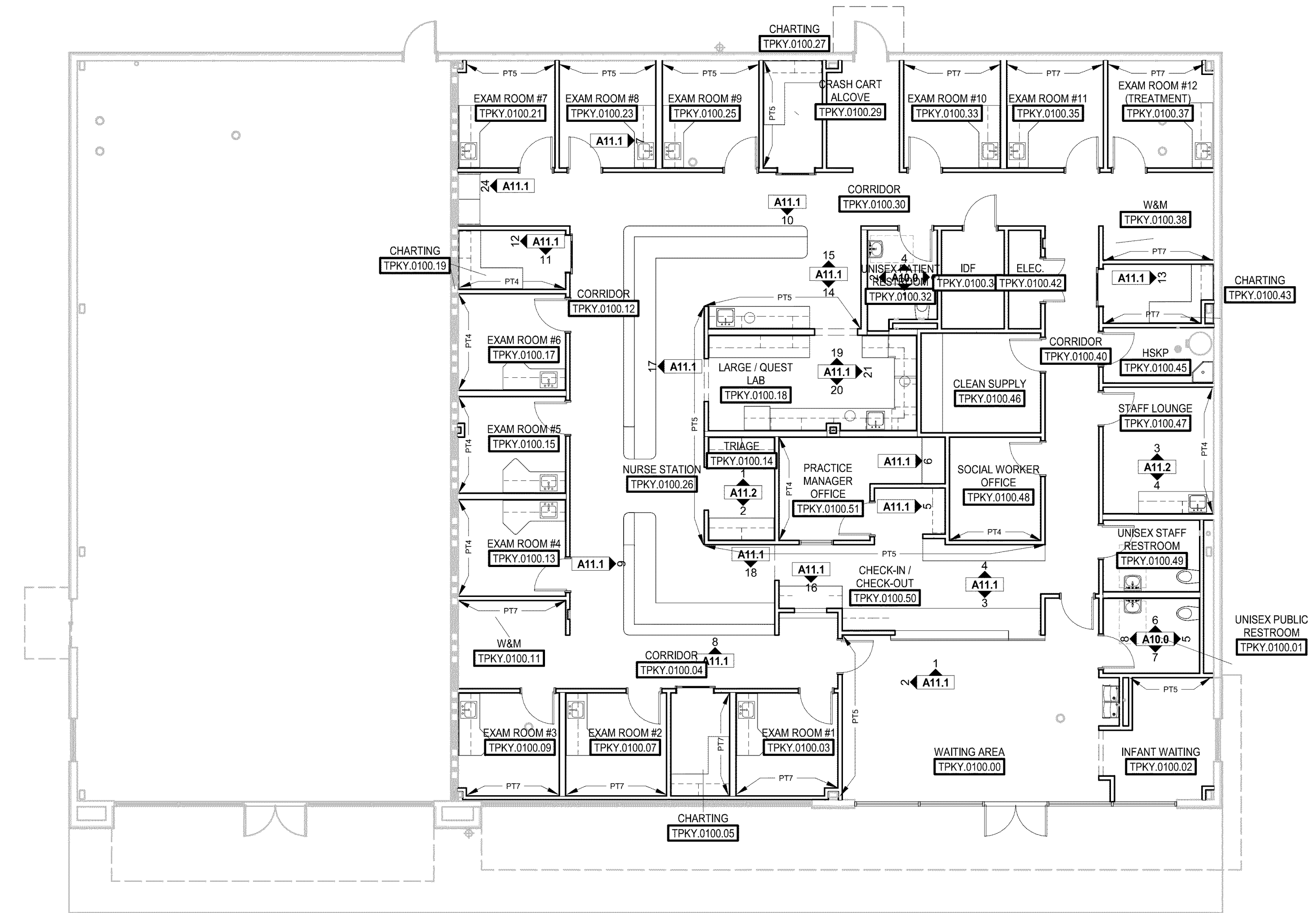
2 FIRST FLOOR WALL FINISH PLAN SCALE: 1/8" = 1'-0"
